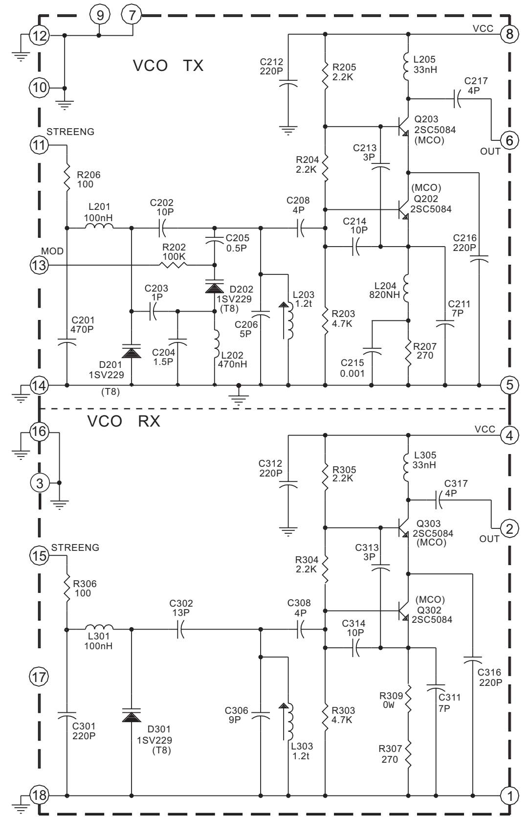
V.C.O. (440-470MHz) 770-030-0023
