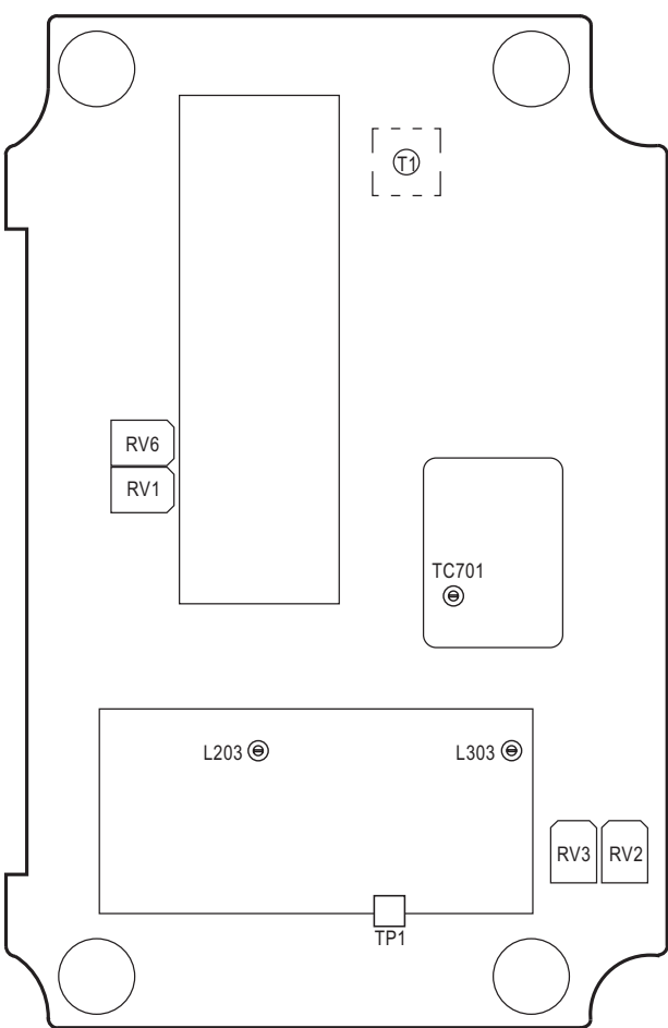
RF BOARD ALIGNMENT POINTS
