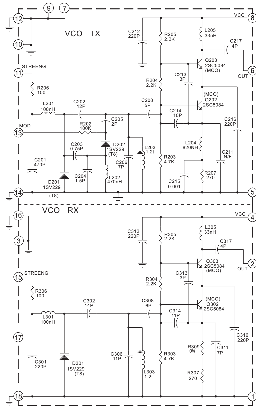
V.C.O. (400-430MHz) 770-030-0026
